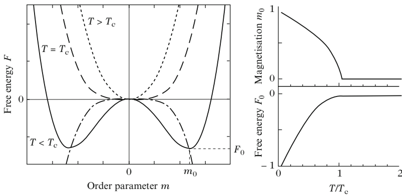
Fig. 1.24 Solutions to Landau's theory in the absence of external field for a homogeneous system
