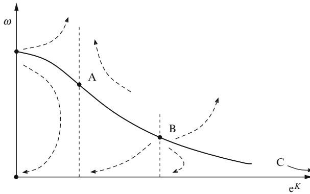
Fig. 6.9 Renormalisation flow in (e^K, \omega) parameter space. Point A is associated with the universality class of self-avoiding walks (scaling law R(N) \sim N^\nu ), point B corresponds to the \Theta point (scaling law R(N) \sim N^{\nu_\Theta} ) and point C , pushed back to infinity with the choice of coordinates (e^K, \omega) , corresponds to the globular phase (scaling law R(N) \sim N^{1/d} )
