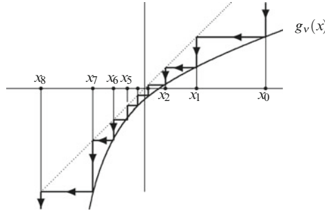
Fig. 9.12 Graph (bold line) of a map g_v parametrised by v and conjugated to the normal form f_\mu(x) = -\mu + x - x^2 . The figure explains how slow and monotonous the discrete evolution x_{n+1} = g_v(x_n) is if v is slightly above a value v_c associated with a saddle-node bifurcation at a fixed point x^* (here placed at the origin) characterised by g'_{v_c}(x^*) = +1
