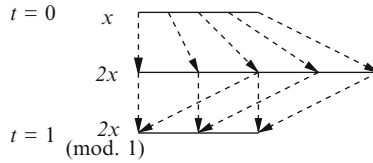
Fig. 9.9 Expansion by a factor of 2 and folding superimposing images of x and x + 1/2 , which is the root of the chaotic nature of the dynamics generated by the transformation x \rightarrow 2x (modulus 1)
