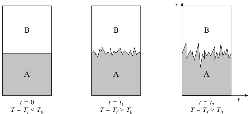
Fig. 4.4 Self-similarity of a diffusion front, here of a fluid A in an fluid B , miscible only at temperatures T > T_0 . The system is prepared at a temperature T_i < T_0 where the two fluids are not miscible and separate under gravity. The system is then brought to a temperature T_f > T_0 . A complex interface develops: the composition of the mixture shows fluctuations at all scales
