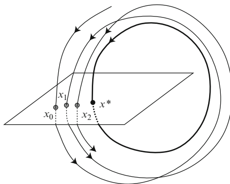
Fig. 9.2 Discretisation by “Poincaré section”. We keep only the trace of a continuous time evolution in a section of phase space transverse to a periodic trajectory (a planetary orbit in Poincaré’s original work), here in bold. Instead of studying a trajectory x(t) , we study the sequence of points of intersection (x_n)_{n \geq 0} with this section. Note that this discretisation is intrinsic to the dynamics (the “first passage time” taken to pass from x_n to x_{n+1} depends on n and the trajectory under consideration). The presence of a periodic trajectory is not an absolutely necessary condition: it is invoked to ensure that neighbouring trajectories will actually recross the chosen section
