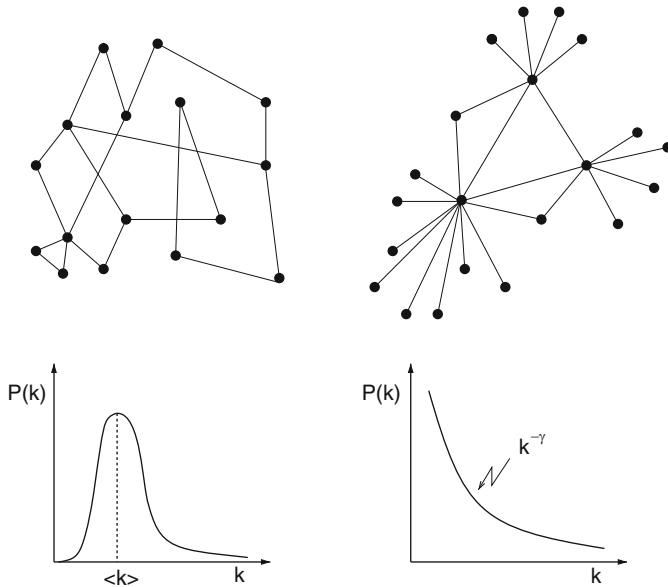
Fig. 11.5 Comparison between random graphs ( left ) and scale-free networks ( right ). Random graphs are relatively homogeneous, whereas in scale-free networks there exist “hub” sites with a large number of connections. Random graphs have a degree distribution P(k) peaked at \langle k \rangle and decaying exponentially, whereas scale-free networks have a power law distribution P(k) \sim k^{-\gamma}
