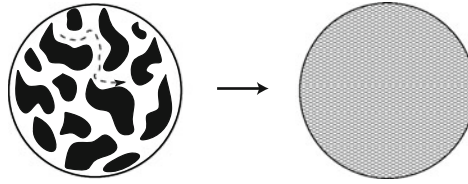
Fig. 4.6 Left: the real porous medium: the intervening space (white) is full of fluid in which diffusion takes place, described by the equation \partial_t c_0 = D \Delta c_0 completed by the boundary conditions, reflecting the fact that the particles, of local concentration c_0(\mathbf{r}, t) , cannot penetrate the solid regions (black), where the concentration is therefore c_0 = 0 . Right: the effective homogeneous medium: we describe the local state by a concentration c = \langle c_0 \rangle , obtained by a spatial average over a representative volume. The diffusion is therefore governed by the equation \partial_t c = D_{\text{eff}} \Delta c . The effective diffusion coefficient D_{\text{eff}} , proportional to D , takes into account in an average way how the diffusion slows down due to the reduction of space actually accessible. Here the diffusion remains normal
