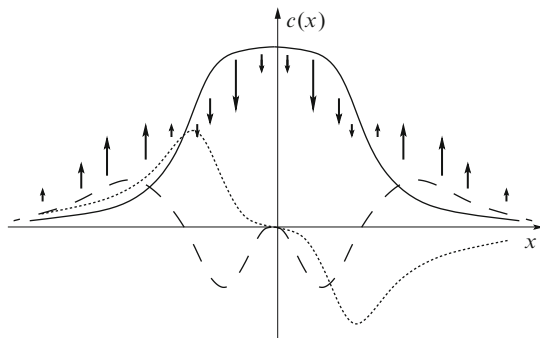
Fig. 4.5 Graphical interpretation of the diffusion equation \partial_t c = D \partial_{xx}^2 c . A localised initial condition c (continuous line), its spatial derivative \partial_x c (dotted line) and the term D \partial_{xx}^2 c (dashed line) – how this term evolves c is shown by the arrows
