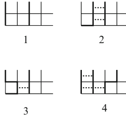
Fig. 6.8 Calculation of the probability \omega_1^2 e^{K_1} of a contact between two renormalised bonds. We have represented a few starting chain configurations similar up to one contact at the level of the renormalised chain. We must exclude counting configurations that will lead to branches or crossings in the renormalised configuration. We obtain: \omega_1^2 e^{K_1} = \omega^4 + 2\omega^5 + 3\omega^6 + e^K \omega^5 (1 + \omega)^2 + e^{2K} \omega^4 (\omega + 2\omega^2 + 4\omega^3 + \omega^4) + 2e^{3K} \omega^7 + e^{4K} \omega^6 (1 + \omega + 2\omega^2) + e^{6K} \omega^8
