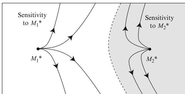
Fig. 3.12 Line separating the zones of influence of two fixed points
