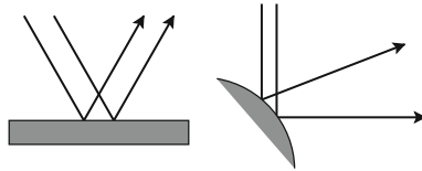
Fig. 9.7 Sensitivity to initial conditions. The phase space is here real space (the surface of a billiard or pool table) but the idea generalises to trajectories in an abstract phase space. Left : bouncing off a flat surface conserves the difference between the incident trajectories. Right : bouncing off a convex surface amplifies the difference between incident trajectories by a factor increasing with the curvature of the obstacle
