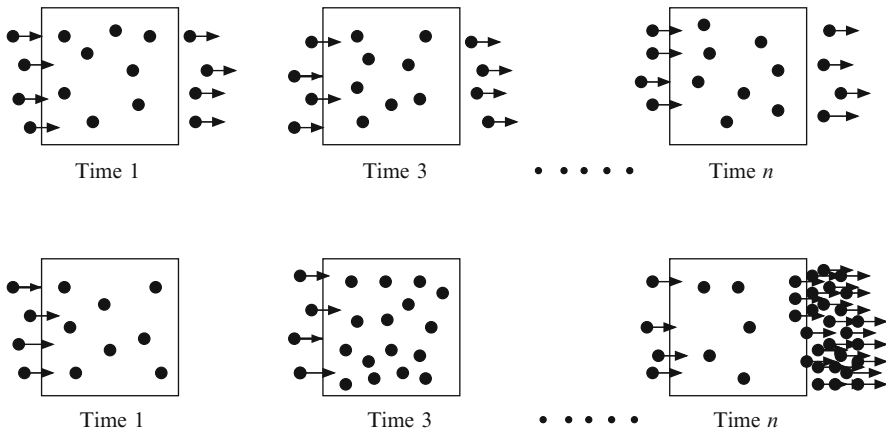
Fig. 10.4 Temporal asymmetry of flows entering and leaving in self-organised criticality ( lower section of figure ). Even though the average values of these flows on very large timescales are equal, there is a slow accumulation of energy or constraints, over n \gg 1 time steps, and very fast relaxation in a single time step. This mechanism, related to the existence of a stability threshold in the local dynamics, contrasts with the case of “dynamic equilibrium” ( upper section of figure ) where flows equilibrate in short timescales and produce a “normal” steady state
